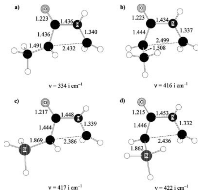
Figure 1. B3LYP/6-311+G(d,p)-optimized geometries of the transition states for the electrocyclic conrotatory closure step for the reactions between methylketene and formaldimine by a) the anti and b) the syn approaches, and between silylketene and formaldimine by c) the anti and d) the syn approaches. Lengths are given in Ångströms.
