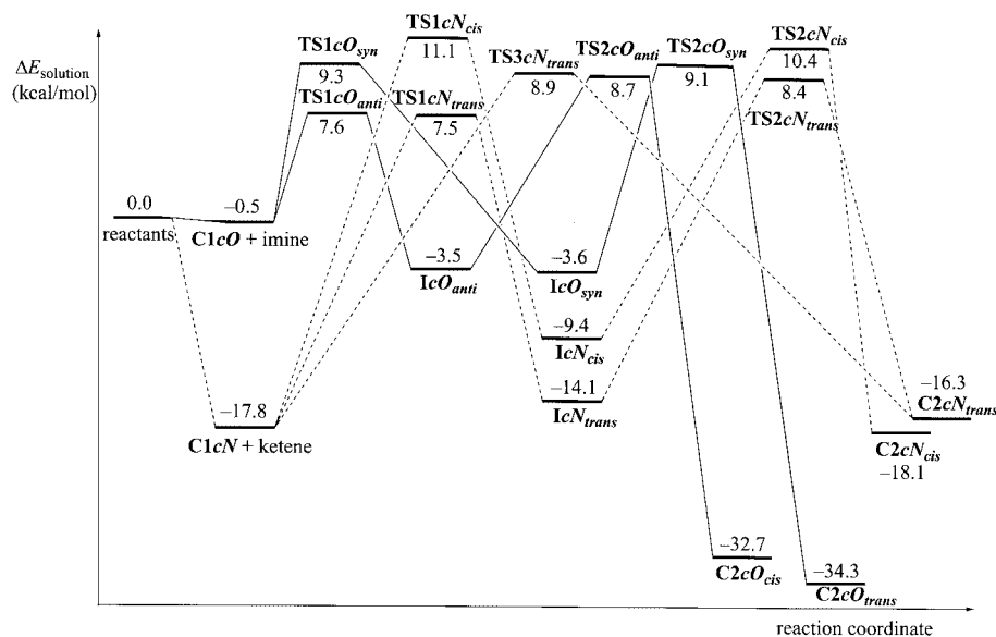
Figure 2. B3LYP/6-311+G(d,p)/PCM//B3LYP/6-311+G(d,p)/Onsager+ZPVE(B3LYP/Onsager) energy profiles for the reaction between silylketene and trans -(methoxycarbonyl)- N -methylformaldimine in the presence of \text{BF}_3 .
